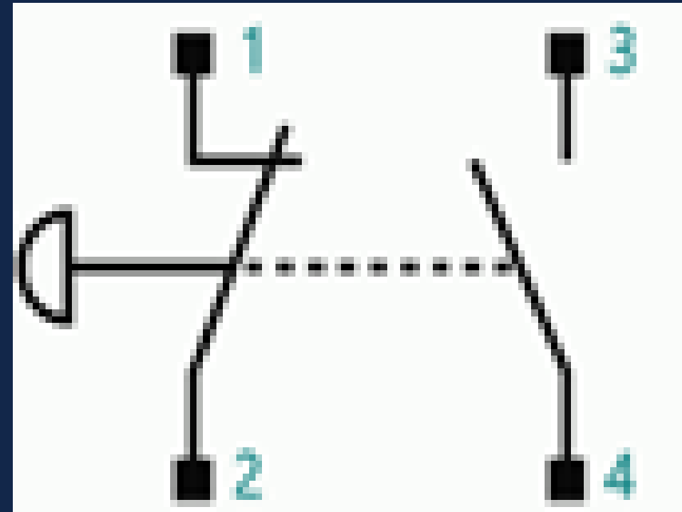
Simbol Emergency Stop
