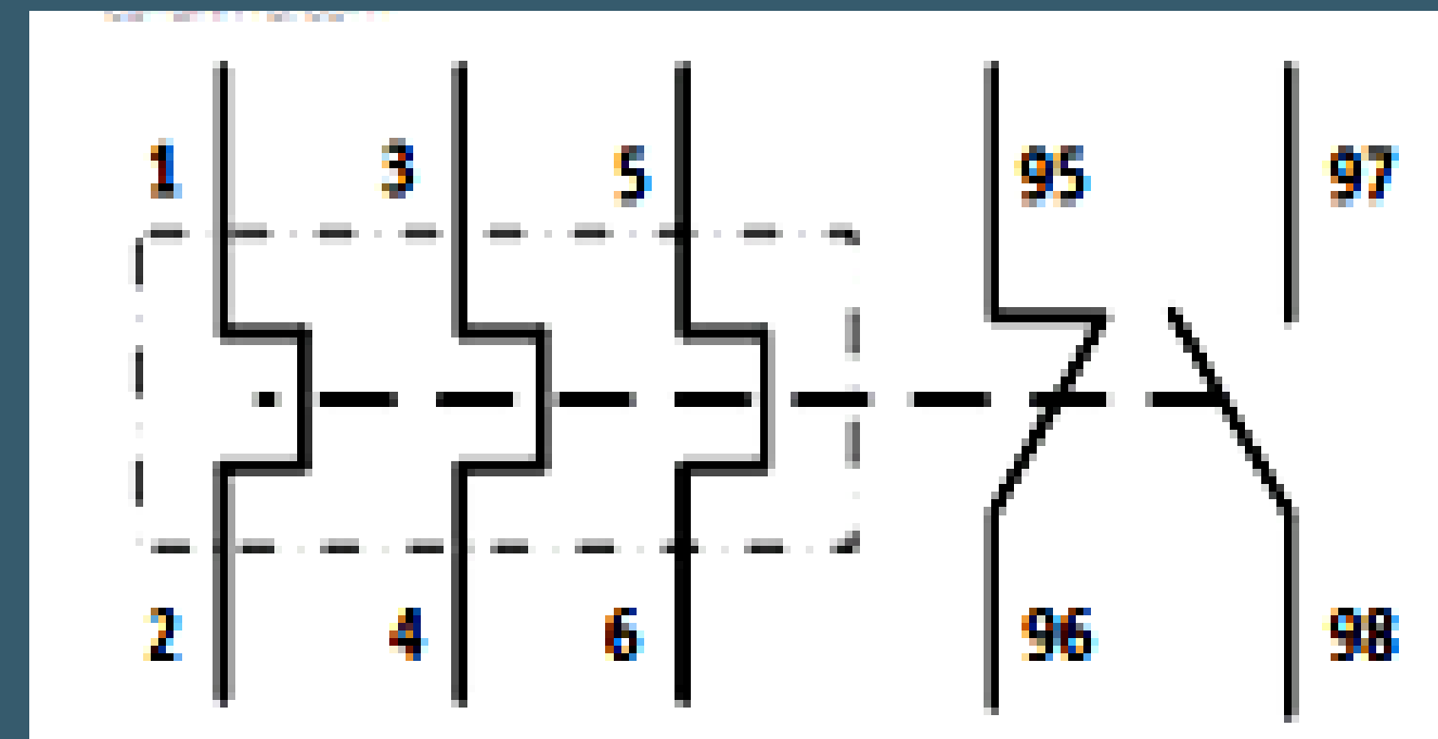
Simbol TOR
