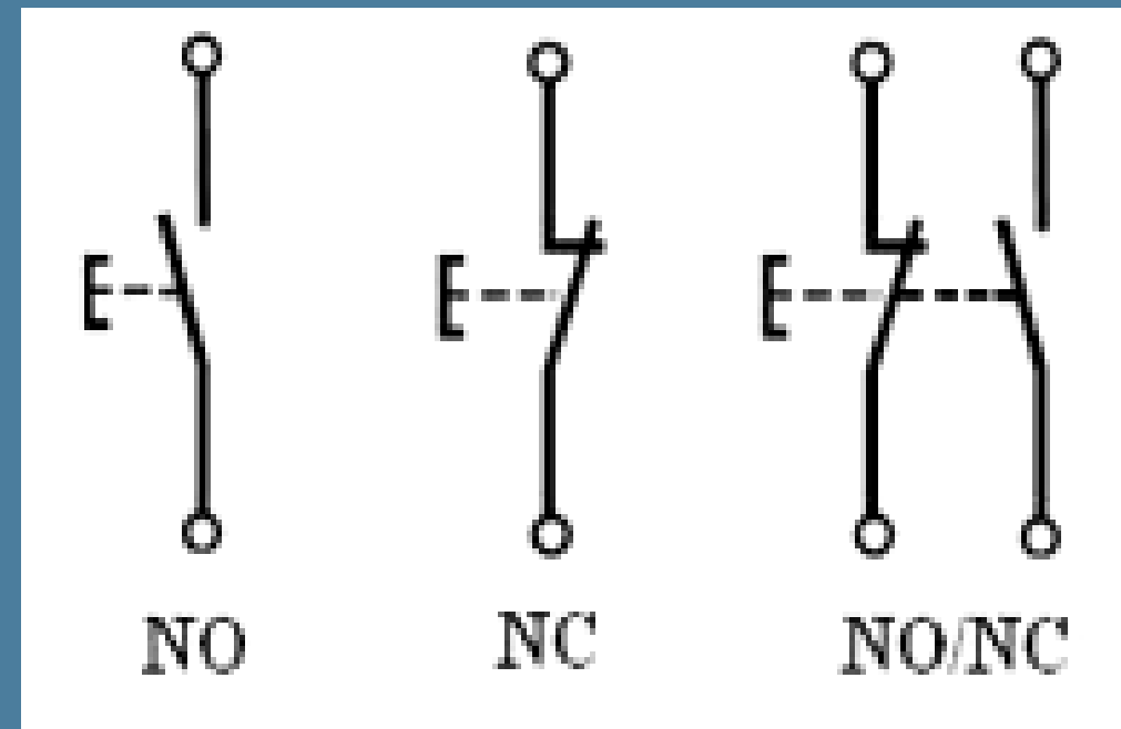
Simbol Push Button
