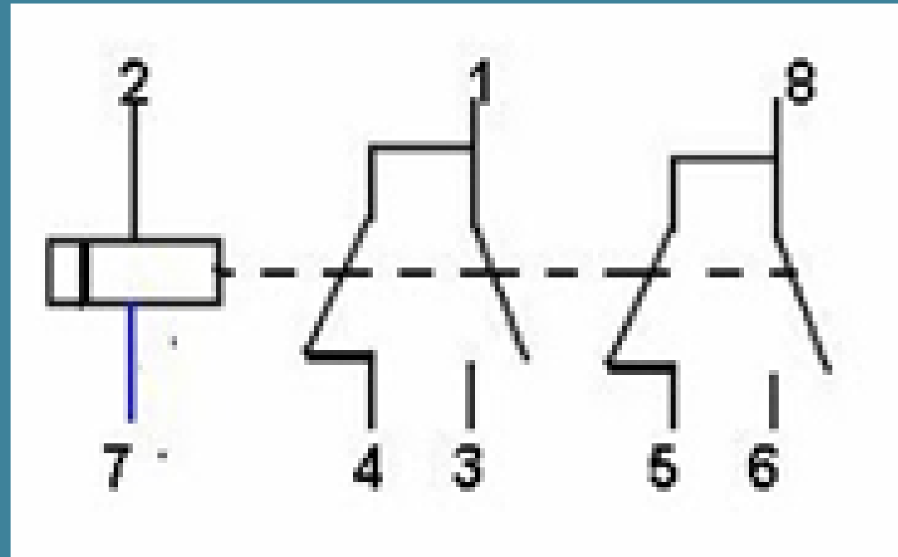
Simbol TIMER
